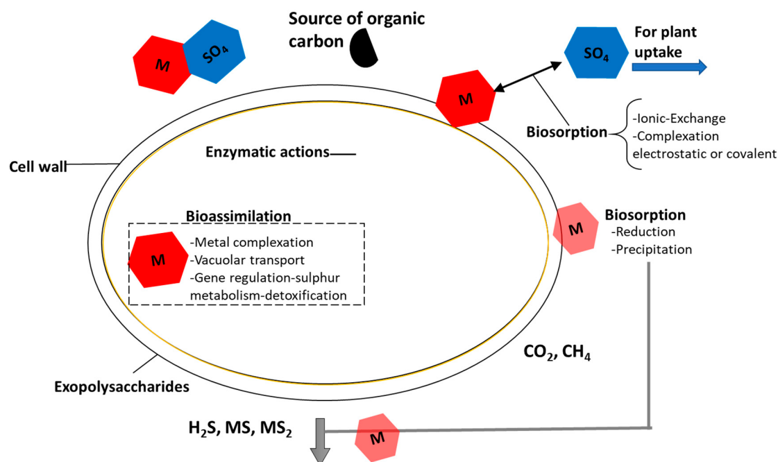
Figure 3. Possible mechanisms of bacteria present in constructed wetlands for the removal, transformation, and tolerance of heavy metals in acid mine drainage (AMD).
