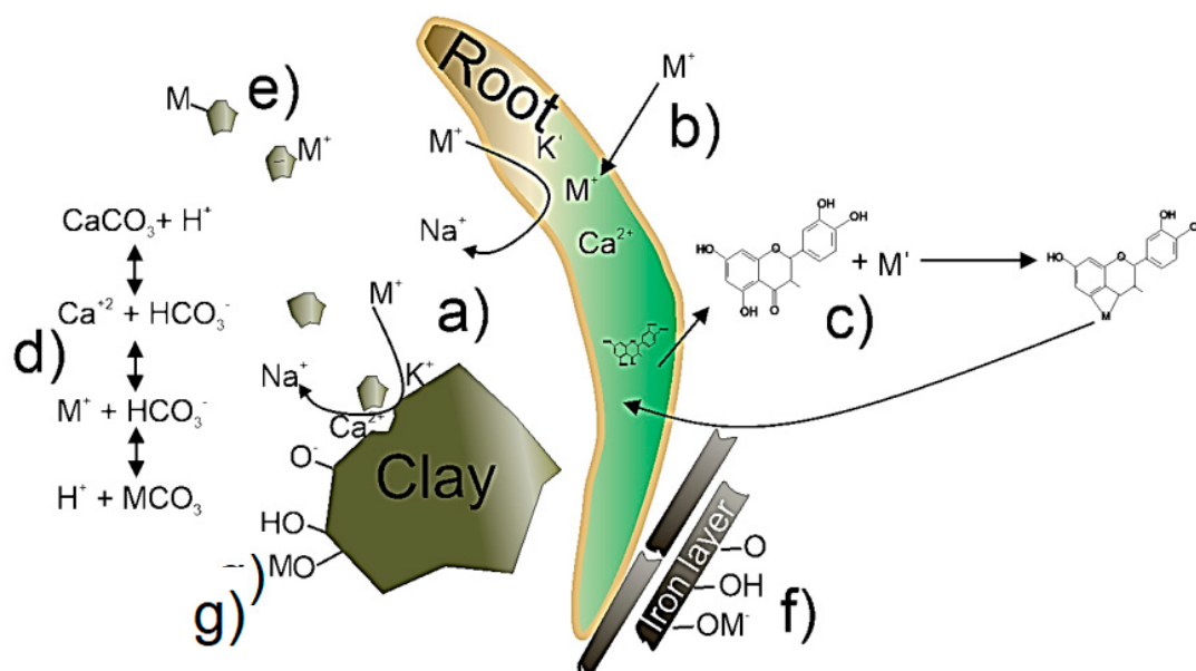
Figure 2. Metal removal mechanisms in constructed wetlands by plant and support material. (a) cation exchange; (b) plant uptake; (c) metal chelation by root exudates; (d) carbonate precipitation; (e) adsorption to particulate matter; (f) adsorption onto iron layer and (g) adsorption onto clay material.
