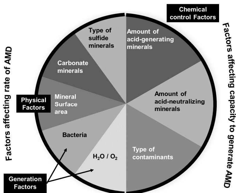
Figure 1. Factors that influence the formation of acid drainage.
